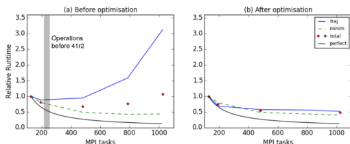
Fig. 2. Scalability of the 4D-Var trajectory (traj) calculation and minimisation (minim) across MPI tasks before (a) and after (b) optimisation. ‘41r2’ refers and grey-shaded area refer to performance at operational model allocation. More details are in the text.
