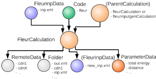
Fig. 1. Database input and output nodes in the directed acyclic provenance graph for a single run of the FLEUR code.
