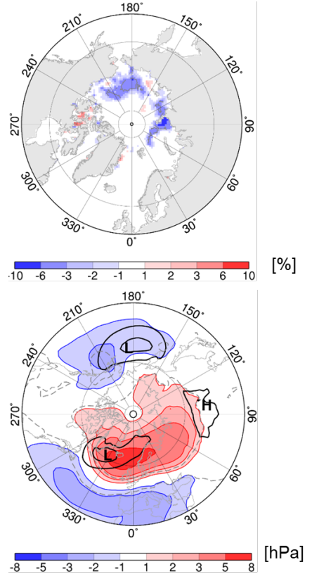
Fig. 3. Coupled patterns obtained by MCA of HadISST1 sea ice concentration (SIC) in September with ERA-Interim SLP in the following February from 1979 to 2015. The leading MCA patterns explain 39% of the squared covariance fraction. The SIC anomaly maps (top) are shown as heterogeneous regression map, the corresponding anomaly map for SLP (bottom) as homogeneous regression maps. Thin grey contours show the significance of the regressions at the 95% level. Black contours show the climatological mean (1980–2015) field of SLP. All data have been linearly detrended before calculating the MCA.
