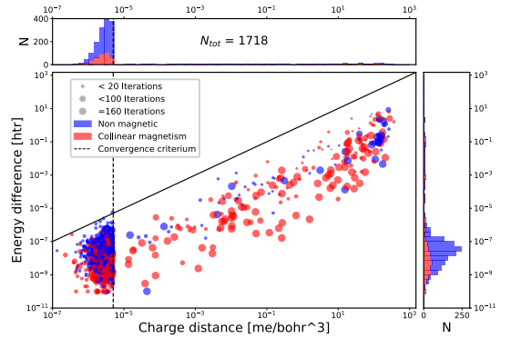
Fig. 3. Small example of the charge density and total energy convergence result of 1718 different binary crystal systems managed by the FLEUR self-consistent field workflow. The workflow succeed in over 86 % of the simulations to fully converge the systems.
