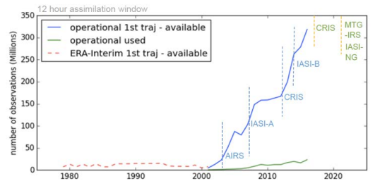
Fig. 1. Time series of observations received by ECMWF within 12 hours. Total number (blue), used number after screening (green) and total number in ERA-Interim reanalysis prior to 2001 [4]. Note volume boosts produced by spectrometer-type instruments such as the Atmospheric Infrared Sounder (AIRS), the Infrared Atmospheric Sounding Interferometer (IASI), the
