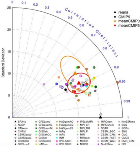
Fig. 2. Taylor plot to quantify similarity of the NAO pattern simulated by CMIP5 models and ERA40 and NCEP/NCAR reanalyses data. Ensemble mean and spread are indicated for the CMIP3 (orange) and CMIP5 ensembles.
